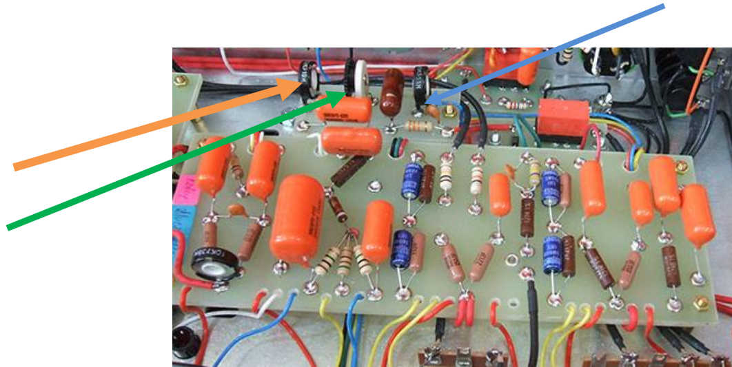
Internal view of Bluesmaster 100W illustrating post-overdrive tonestack. ORANGE arrow is MIDRANGE GREEN arrow is BASS BLUE arrow is TREBLE
