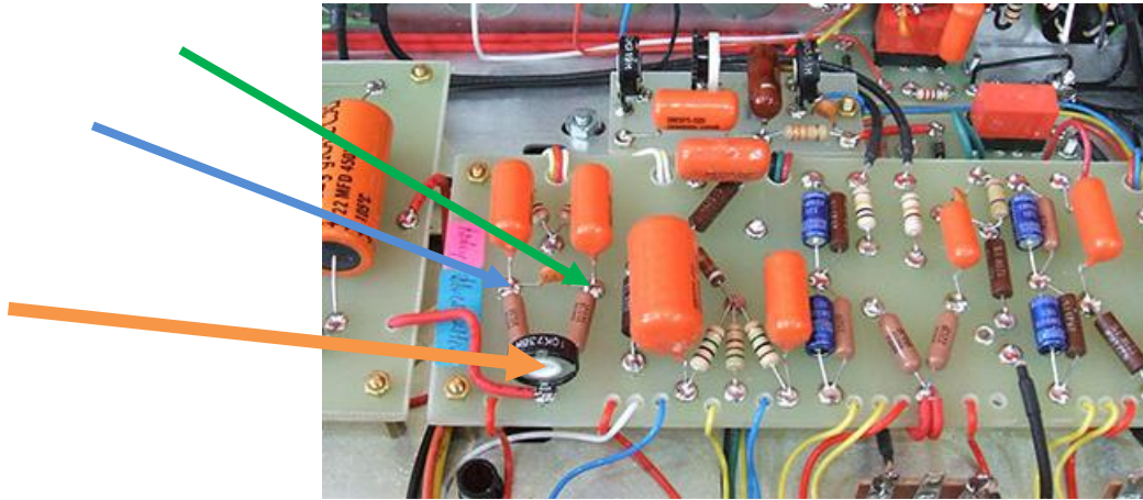
Inside chassis view of Bluesmaster 100W. Orange arrow indicates PI trimmer. Blue arrow indicates V3B test point Green arrow indicates V3A test point.
